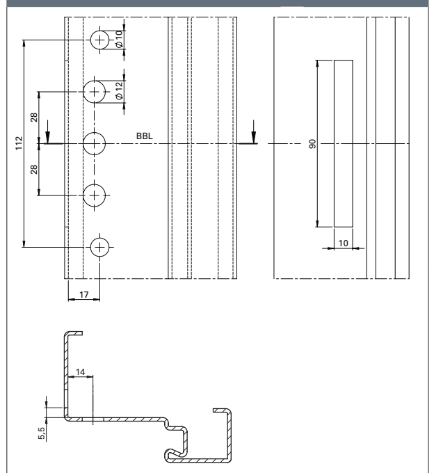
Hole pattern
