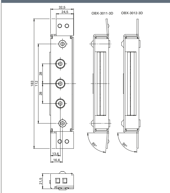
Dimensional drawing
