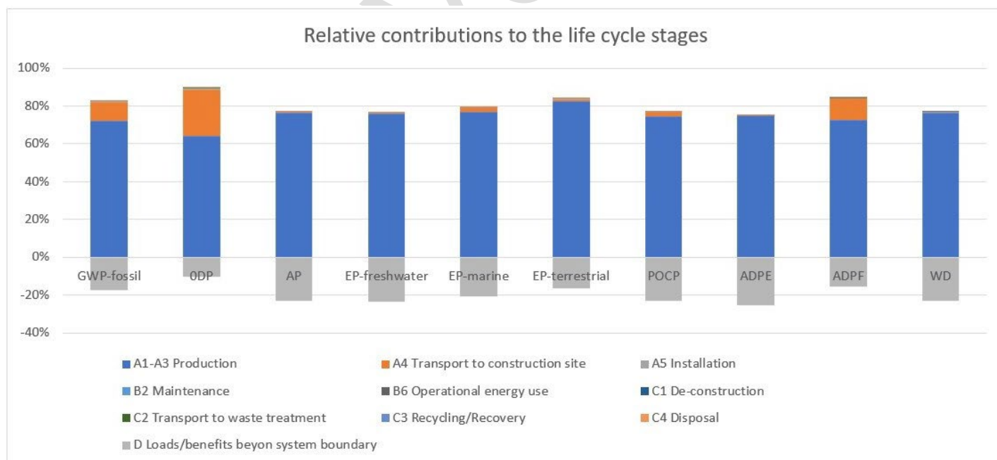
Figure 1: Environmental impacts of door and window handles (Ha) along its life cycle
