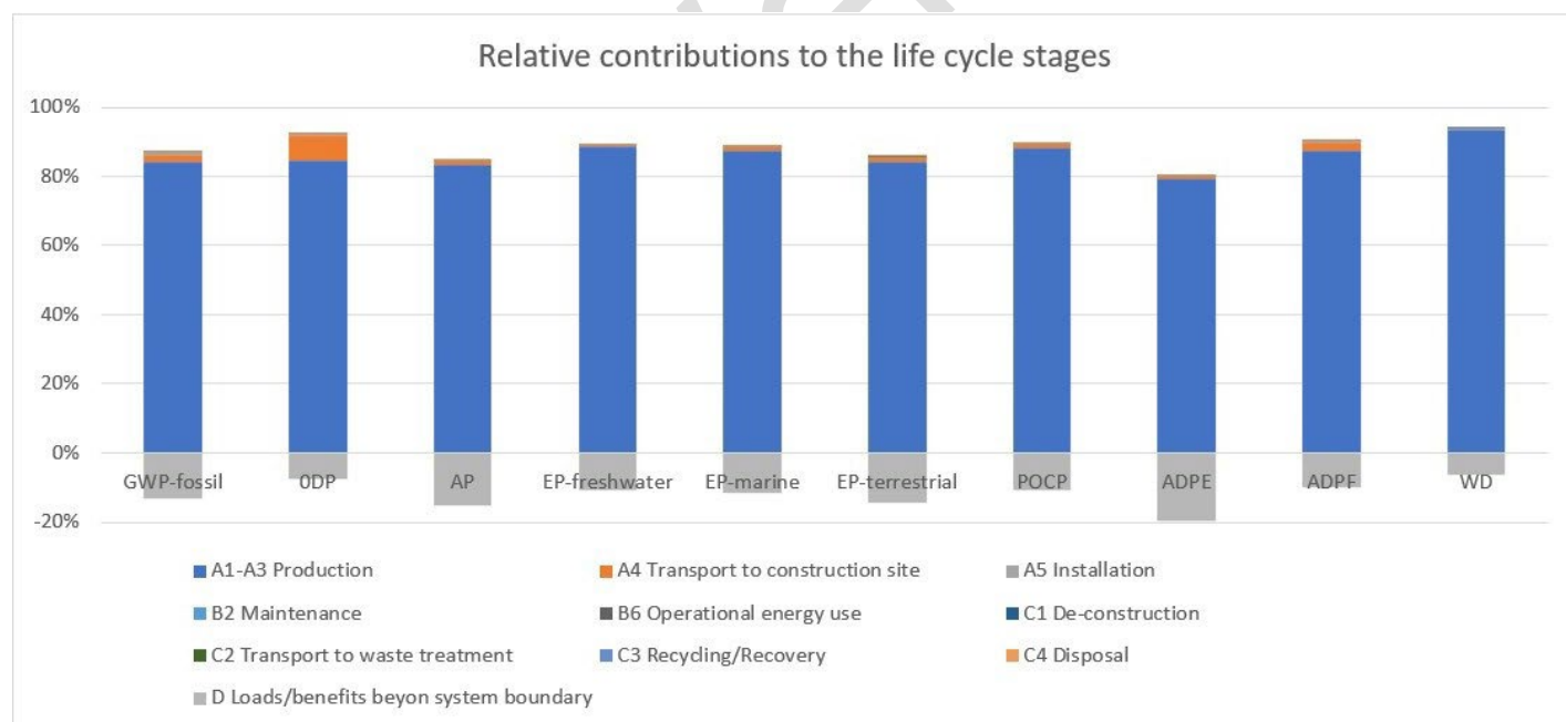
Figure 1: Environmental impacts of door closers (DC) along its life cycle
